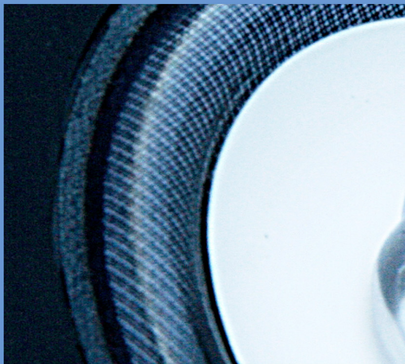
Detail surround met super dun (0,09mm) keramisch inverted dome-membraan
